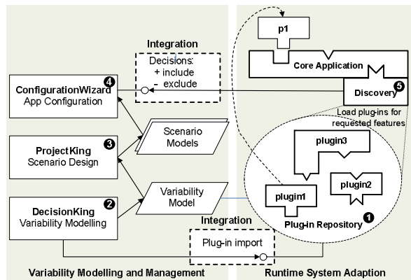
Fig. 2: Integration of PLE tools and plug-in techniques to support runtime adaptation.
