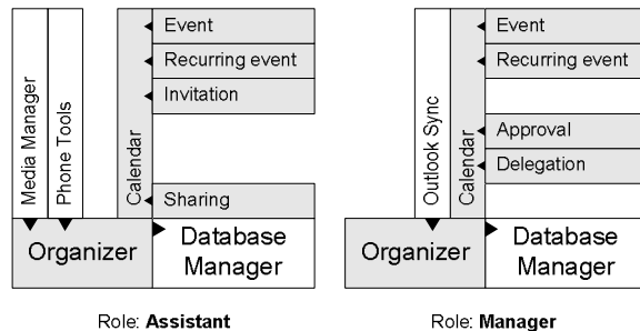
Fig. 9: Loaded plug-ins for the roles Assistant and Manager.
