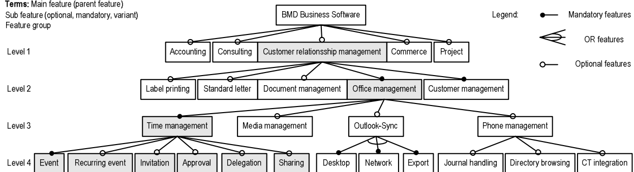
Fig. 6: Partial BMDCRM feature model.
