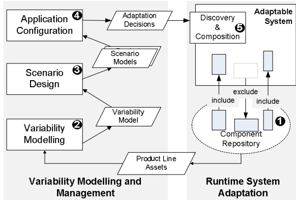
Fig. 1: Integrating variability management, configuration, and adaptation techniques.
