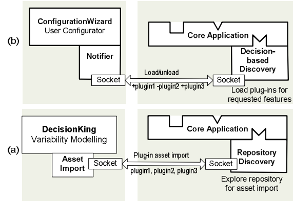
Fig. 5. Integration: (a) asset import, (b) decision-based discovery and activation.
